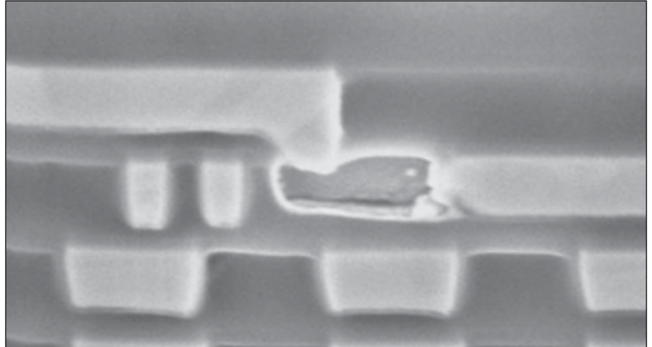
Figure 1: A scanning electron microscopy image of a copper line interconnect where a void has developed due to vacancy accumulation. This has led to a broken circuit.
