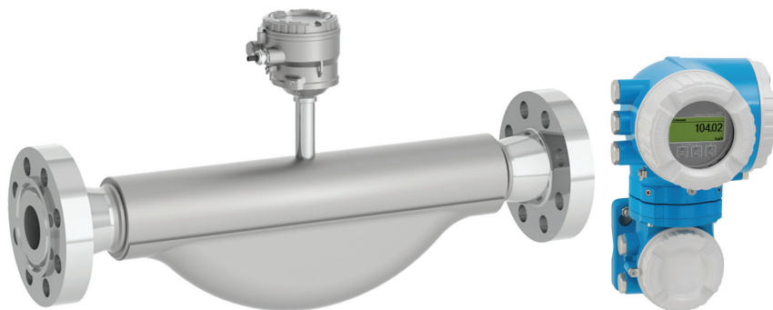
FIGURE 1. Coriolis flow meter designed at Endress+Hauser.
