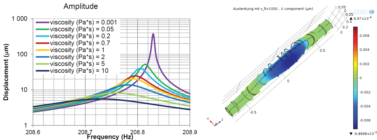
FIGURE 3. Simulation results showing the change in tube oscillating frequency for different fluid viscosities and the resulting mechanical displacement. At right is a visual example of tube deformation due to the oscillating motion.
