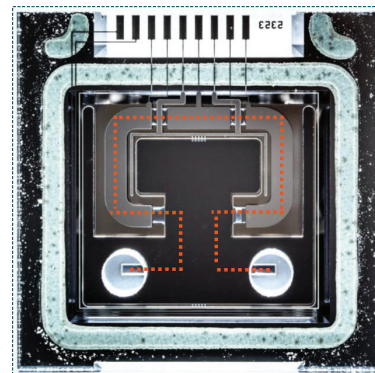
FIGURE 4. MEMS Coriolis chip used for density and viscosity measurements. Left: Complete sensor held by pliers. Right: Chip layout inside the device.
