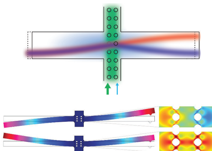
FIGURE 2. Schematic (top) and simulation (bottom) of an optomechanical atomic force microscope (AFM) that takes advantage of optical cooling. Credit: Xu et al./NIST and University of Maryland.
