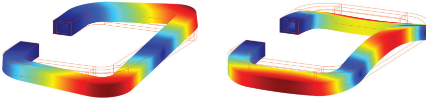
FIGURE 5. Two eigenmodes of the oscillating microchannel. Color denotes the relative displacement levels of different regions of the channel.
