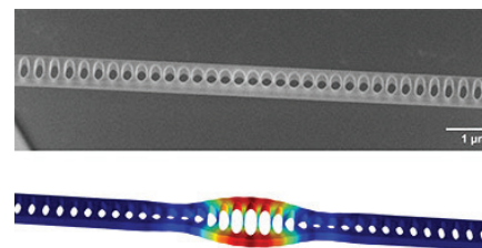
FIGURE 1. Top is an electron micrograph of a silicon nitride beam. The bottom shows how the beam deforms as it vibrates. Credit: Purdy et al., NIST/JQI.
