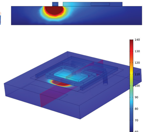
FIGURE 6. Thermal results showing temperature in the MEMS Coriolis chip.
