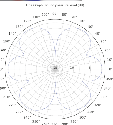
FIGURE 2. Simulation showing the acoustic field in and around the oscillating tube (top and center) and a sound pressure level plot in dB (bottom).
