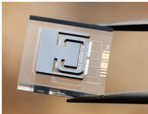
FIGURE 4. MEMS Coriolis chip used for density and viscosity measurements. Left: Complete sensor held by pliers. Right: Chip layout inside the device.
