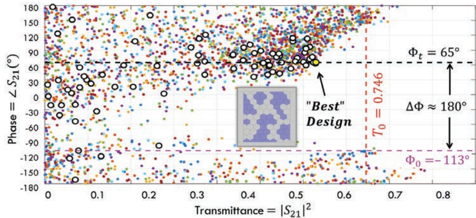
FIGURE 4. Plot of the transmittance, or the scattering parameter |S_{21}|^2 , against the phase. Generations are distinguished with color.
